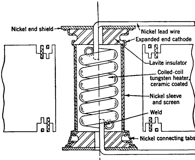
FIG. 12-25.—Metallized screen cathode of the 4J70. (2×.)
